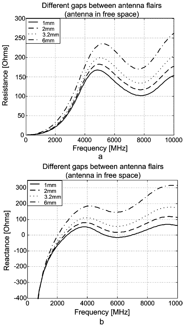
Fig. 4. Input impedance of the butterfly antenna (flair dimension of 20 \times 22 \text{ mm}^2 ) in free space for different widths of the feeding gap: (a) antenna resistance and (b) antenna reactance.
