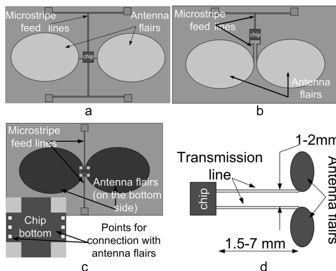
Fig. 8. Three scenarios of RF chip integration with an antenna: (a) chip is located between the antenna flairs, (b) chip is placed below the antenna flairs, (c) chip is placed on the opposite side of PCB, and (d) the feeding line in scenario 2.
