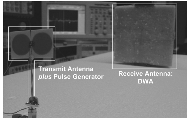
Fig. 17. Measurement setup: (left) butterfly antenna with the integrated impulse generator and (right) dielectric wedge antenna.
