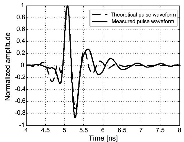
Fig. 18. Transmitted waveforms: measured and simulated by antenna feeding with 470 ps pulse.
