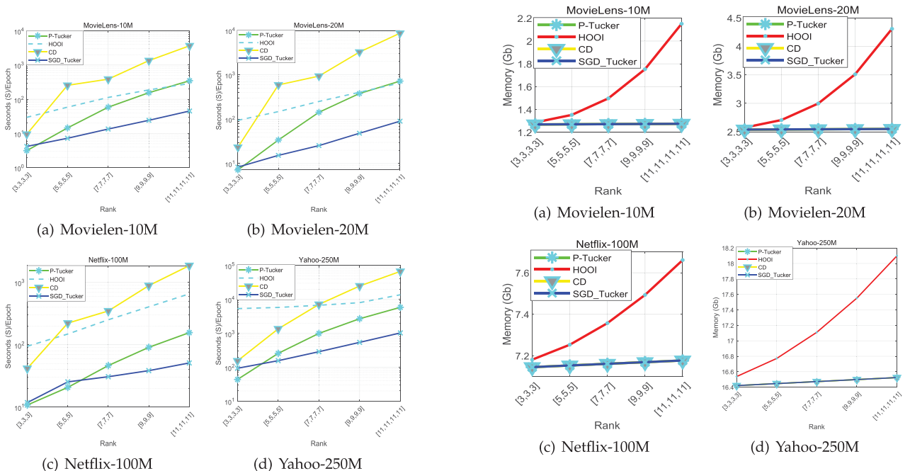
Fig. 6. Rank scalability for memory overhead on a thread running. (In this work, GB refers to GigaBytes and MB refers to Megabytes). The space scalability for P-Tucker, CD, HOOI, and SGD_Tucker on the 4 datasets with successively increased total elements, i.e., Movielens-10M, Movielens-20M, Netflix-100M, and Yahoo-250M.
