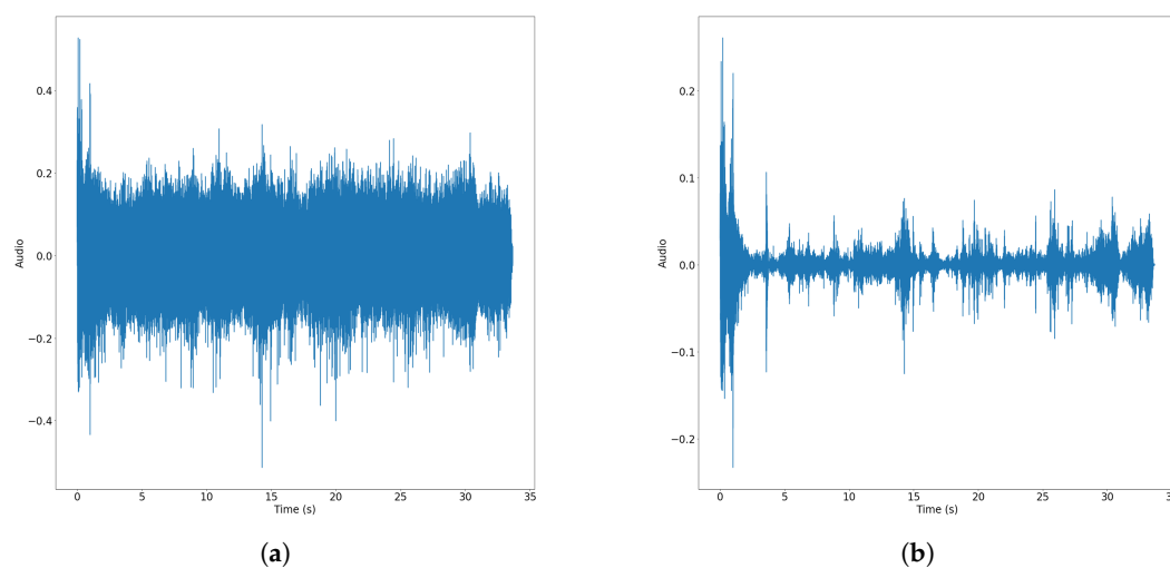
Figure 7. Raw and filtered audio signals from deposition of Invar 36 bead—(a) Raw audio data; (b) Spectral gating-denoised audio signal with threshold = 1.
