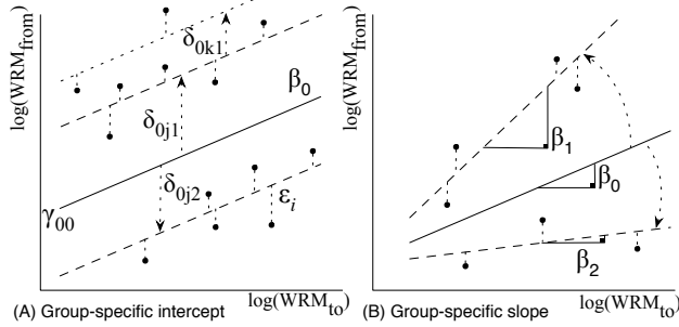
Fig. 9. Visual representation of group-specific intercept and slope. In figure A, the intercept is allowed to vary but regression lines stay parallel; the total group-specific intercept is \gamma_{00} + \delta_{0j} + \delta_{0k} . In figure B, slopes are allowed to vary, leading to a different \beta per group.
