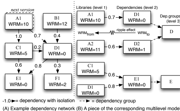
Fig. 7. An example of libraries and their dependencies. On the right side, the corresponding multilevel representation of the left side is shown. Not all nodes and relationships from panel A are included in panel B.
