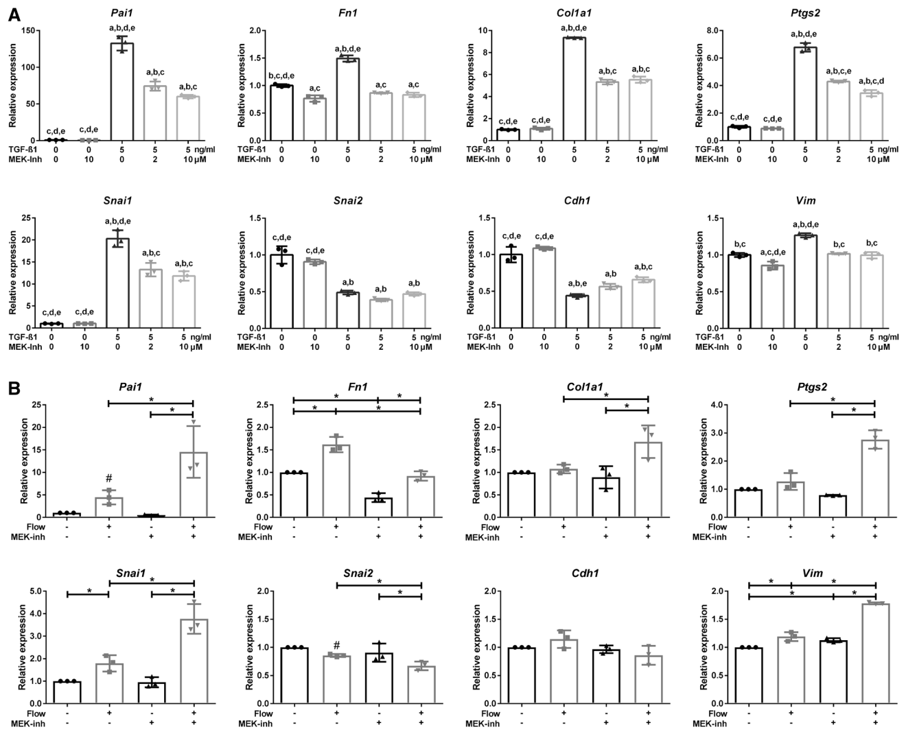
Fig. 6 MEK inhibition modulates fluid shear-induced and TGF- \beta 1-stimulated expression of SMAD2/3 target genes. a MEK inhibition (Trametinib, GSK1120212) reduces TGF- \beta 1 increased expression of Pai1 , Fn1 , Col1a1 , Ptgs2 , Snai1 , and Vim , while expression of Cdh1 is less decreased. Snai2 expression was not significantly changed upon MEK inhibition. Relative mRNA expression measured at t=4 h; n=3 ; Hprt served as housekeeping gene to correct for cDNA input; data normalized to unstimulated controls. Significant difference ( P<0.05 ) by one-way ANOVA: a compared to 0 ng/ml TGF- \beta 1, b compared to 0 ng/ml TGF- \beta 1 + 10 \mu M MEK-inh, c compared to 5 ng/ml TGF- \beta 1, d compared to 5 ng/ml TGF- \beta 1 + 2 \mu M MEK-inh or
