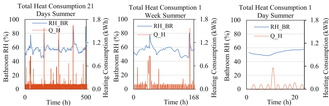
Fig. 4. Total heating consumption, Q_H (in orange) and bathroom RH, RH_BR (in blue) for 21 days of summer. (For interpretation of the references to colour in this figure legend, the reader is referred to the web version of this article.)
