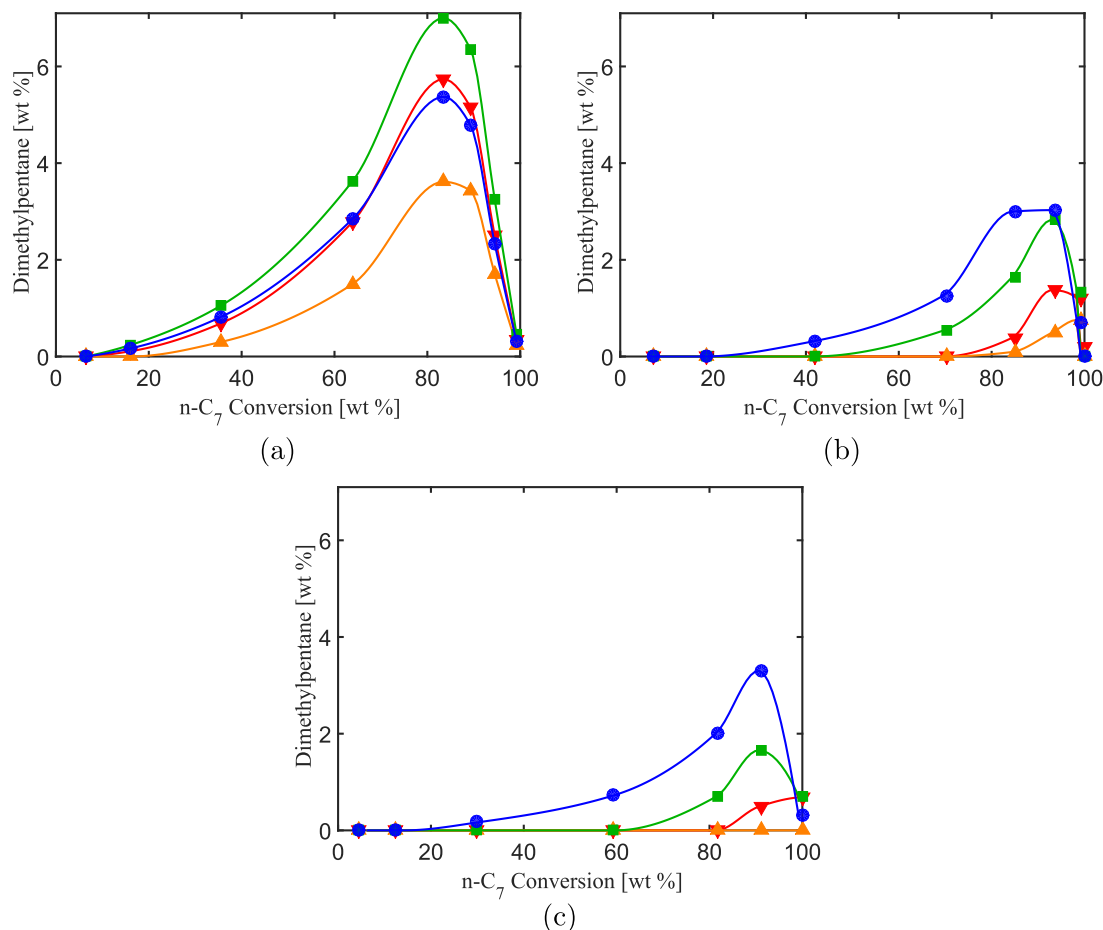
Fig. 6. The experimental yields of dimethylpentanes are plotted as a function of the conversion of n-C 7 for (a) BEA, (b) MFI, and (c) MEL. 23-dimethylpentane (green □), 24-dimethylpentane (blue ○), 22-dimethylpentane (red ▽), and 33-dimethylpentane (orange △). Different conversion levels are obtained by changing the temperature of the reactor between 200 °C and 320 °C. Lines are a guide to the eye.
