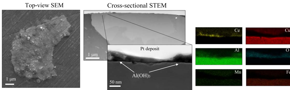
Figure 13. Post-mortem analysis of exposed \text{Al}_7\text{Cu}_2\text{Fe}(\text{Mn}) particles after 96 h. Top-view SEM and cross-sectional STEM/EDS analysis of an \text{Al}_7\text{Cu}_2\text{Fe}(\text{Mn}) particle on an AA2024-T3 sheet exposed to 0.01 M NaCl + 0.003 M \text{Ce}(\text{NO}_3)_3 . The elemental maps correspond to the rectangular region shown in the STEM image. The cross-section has been fabricated with FIB; mind that there is a Pt layer deposited to protect the particle from Ga damage while milling.
