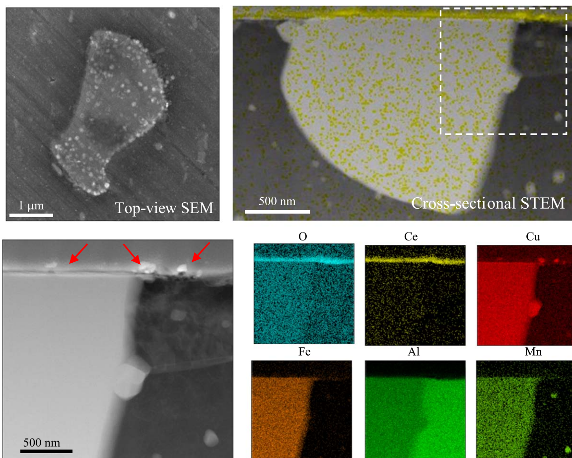
Figure 14. Post-mortem analysis of exposed \text{Al}_7\text{Cu}_2\text{Fe}(\text{Mn}) particles after 96 h. Top-view SEM and cross-sectional STEM/EDS analysis of an \text{Al}_7\text{Cu}_2\text{Fe}(\text{Mn}) particle on an AA2024-T3 sheet exposed to 0.01 M NaCl + 0.003 M \text{Ce}(\text{NO}_3)_3 . The cerium map is superimposed on the STEM image. The elemental maps correspond to the rectangular region shown in the STEM image. The white arrow indicates the Cu nanoparticles deposited on the \text{Al}_7\text{Cu}_2\text{Fe}(\text{Mn}) particle and its adjacent matrix. These Cu nanoparticles cause an enhanced cerium deposition. The cross-section has been fabricated with FIB; mind that there is a C layer deposited to protect the particle from Ga damage while milling.
