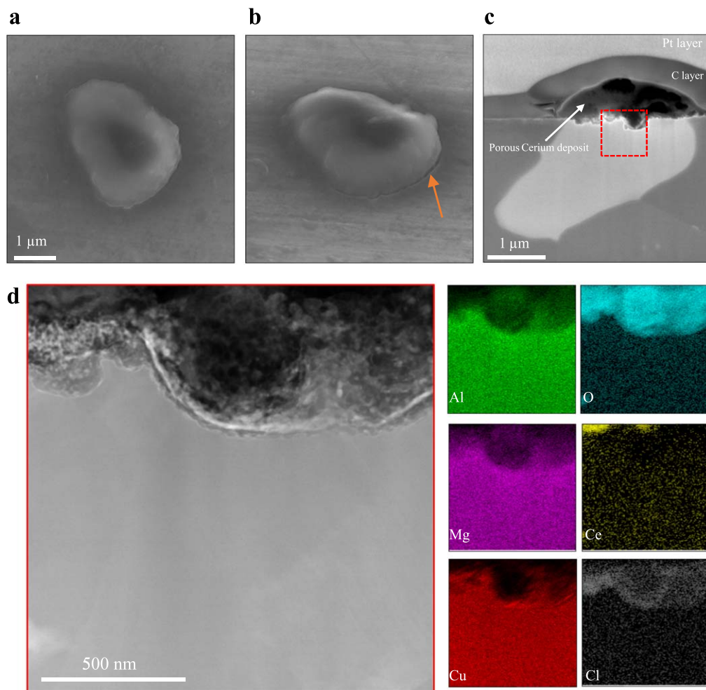
Figure 5. Post-mortem analysis of exposed S-phase particles after 6 h. (a) Top-view SEM of an \text{Al}_2\text{CuMg} particle on an AA2024-T3 sheet exposed to 0.01 M \text{NaCl} + 0.003 M \text{Ce}(\text{NO}_3)_3 . (b) SEM image of the particle when the stage is tilted at 52^\circ ; the orange arrow indicates the gap between the alloy surface and cerium layer. (c) Cross-sectional SEM image of the same particle; the white arrow denotes the porous cerium layer. (d) STEM/EDS analysis of the rectangular region shown in Fig. 5c. The cross-section has been fabricated with FIB. Mind that there is a thin layer of carbon followed by Pt deposition on the particle to protect it from Ga damage while milling.
