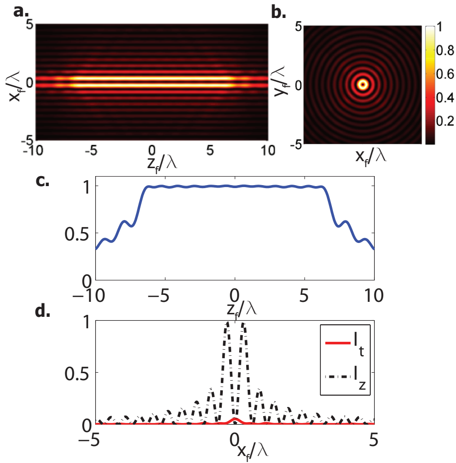
Figure 3: Elongated subwavelength hollow spot by a shaped radially polarized phase vortex with m = 1 on the exit pupil, NA=0.99 . (a).Normalized focal field distribution in the x_f - z_f plane; (b)Focal field in the transversal plane; (c). Focal intensity distribution along the z_f axis, while x_f is at the maximum intensity on the transversal plane (d). Focal intensity distribution along x_f axis.
