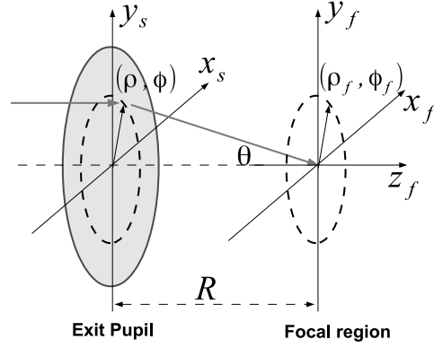
Figure 1: The Debye diffraction model. Light is focused from the exit pupil plane ( x_s, y_s ) to the focal region. The focal coordinates is (x_f, y_f, z_f) with the geometrical focal point as its origin.
