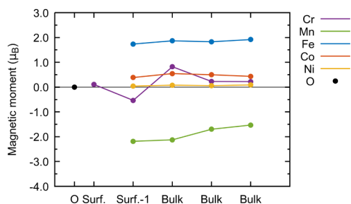
Fig. 6. Converged magnetic moments as a function of position in the slab for the component elements computed with the PAW method in the FM state. The surface layer contains only Cr atoms and is covered by 1 ML of O.
