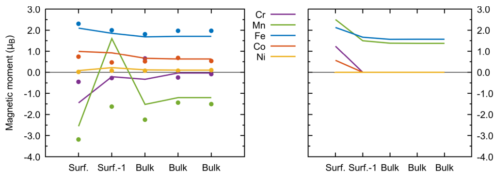
Fig. 2. Converged magnetic moments as a function of position in the slab for the component elements computed with the PAW method (points) and the EMT0 method (lines) in the FM state (left panel) and paramagnetic (DLM) state (right panel, only absolute values of the moments calculated with the EMT0 method).
