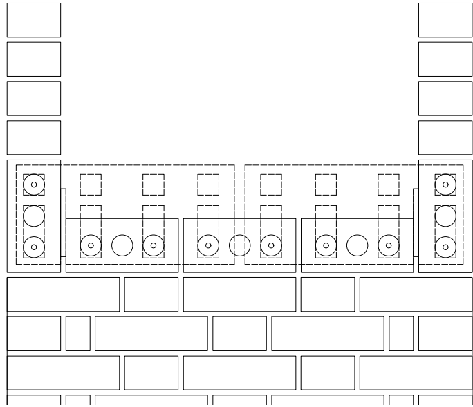
Halfel prefab lintel vertical detail
