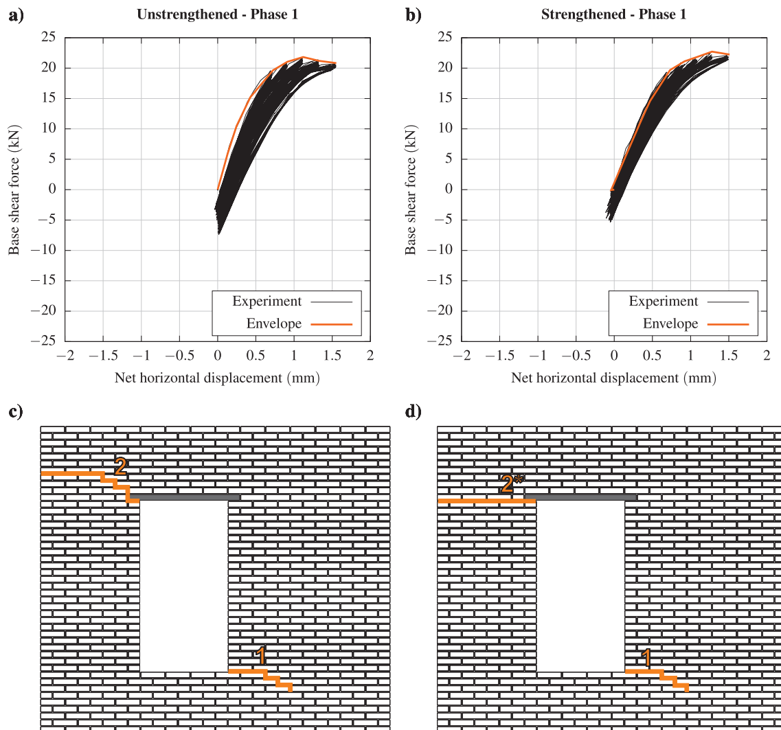
Fig. 4. Experimental results from phase 1: a) force-displacement graph of unstrengthened wall, b) force-displacement graph of strengthened wall, c) crack pattern of unstrengthened wall and d) crack pattern of strengthened wall.
