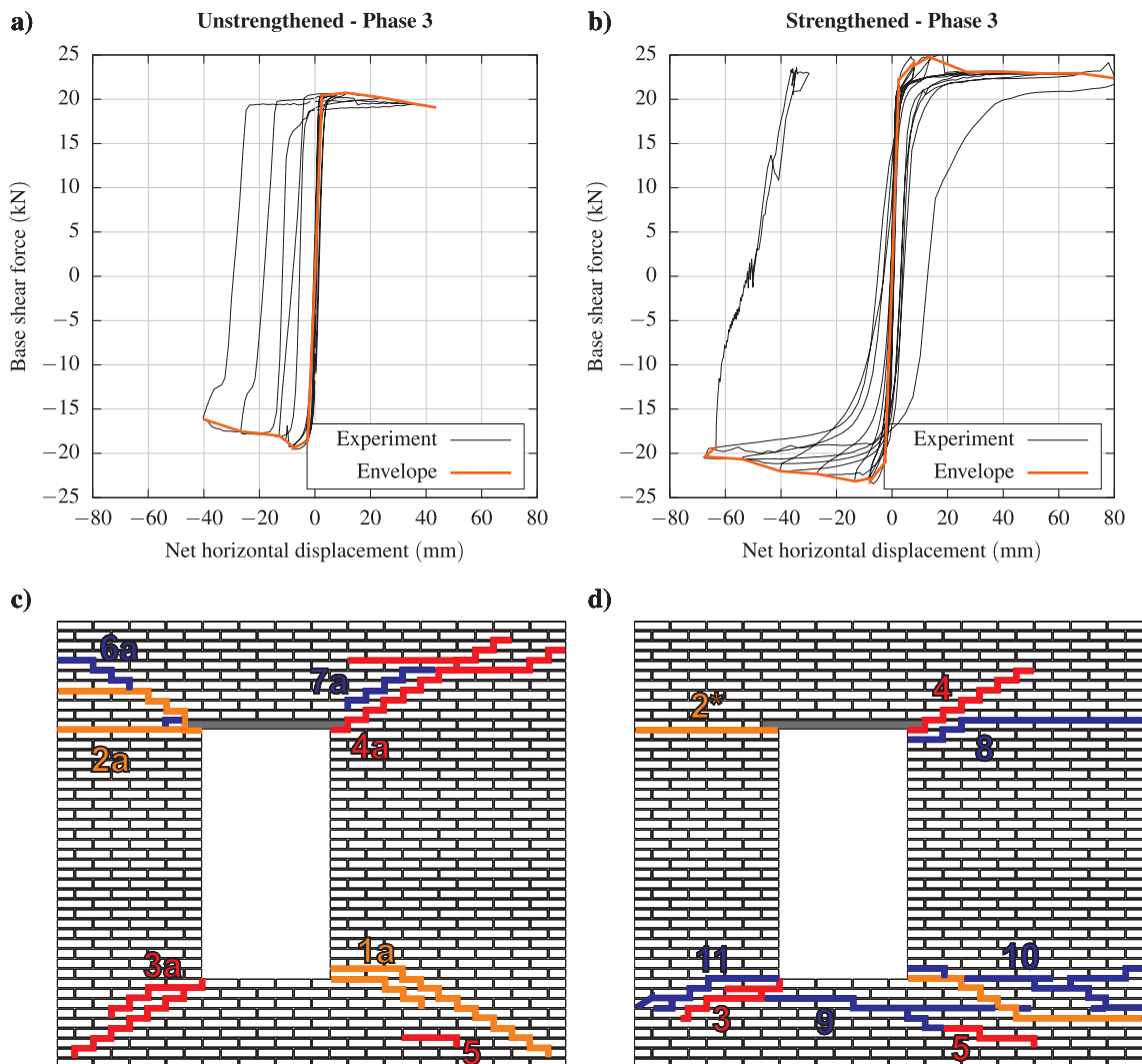
Fig. 6. Experimental results from phase 3: a) force-displacement graph of unstrengthened wall, b) force-displacement graph of strengthened wall, c) crack pattern of unstrengthened wall and d) crack pattern of strengthened wall.
