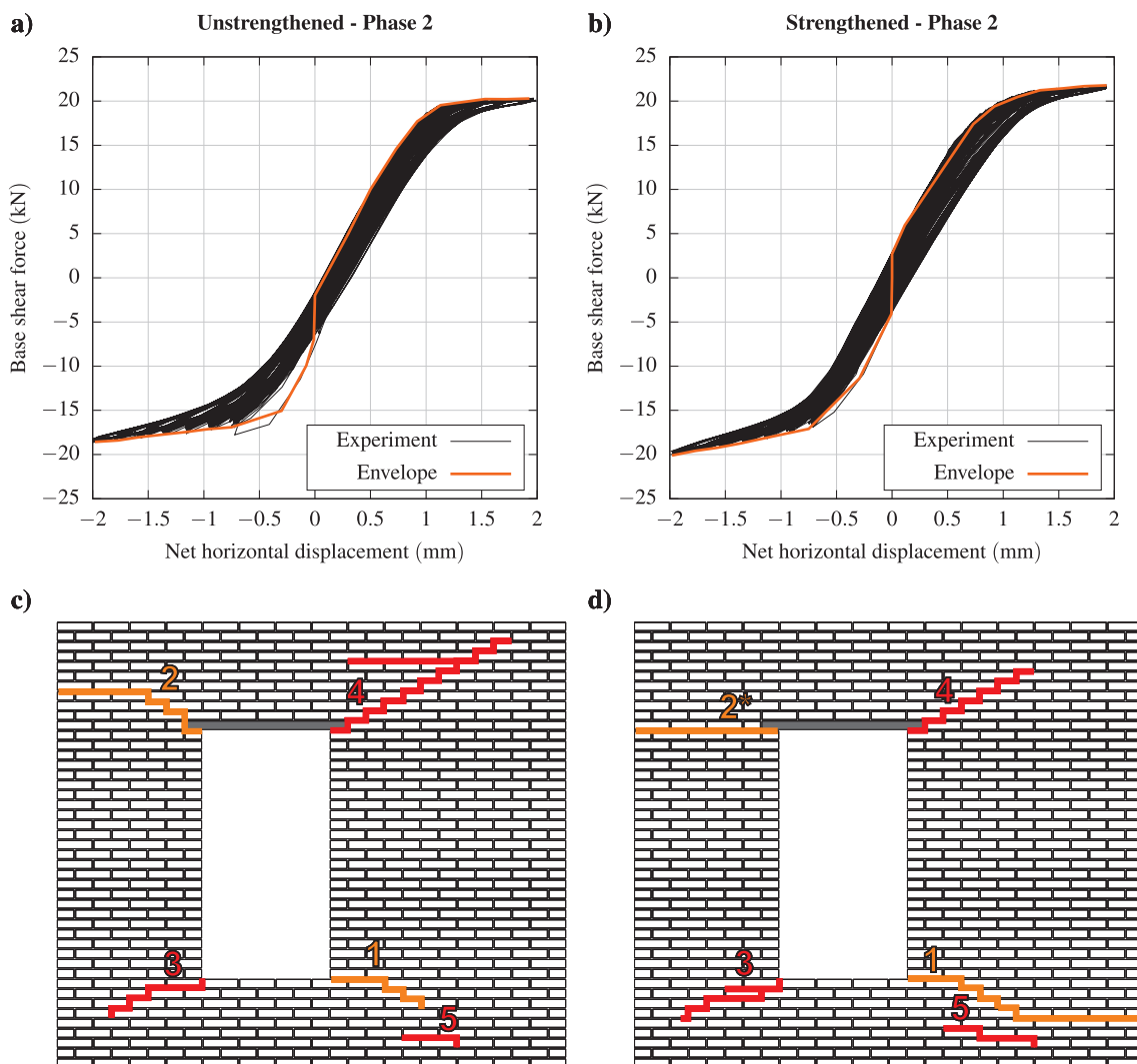
Fig. 5. Experimental results from phase 2: a) force-displacement graph of unstrengthened wall, b) force-displacement graph of strengthened wall, c) crack pattern of unstrengthened wall and d) crack pattern of strengthened wall.
