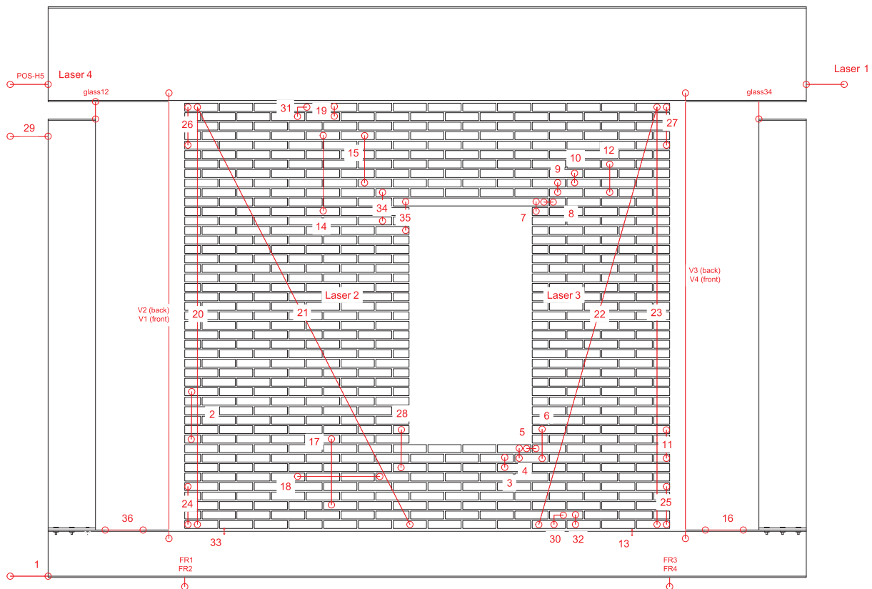
Fig. 2. Sensor layout at the back of the masonry wall for in-plane testing. Placement locations of linear potentiometers and laser sensor targets indicated.
