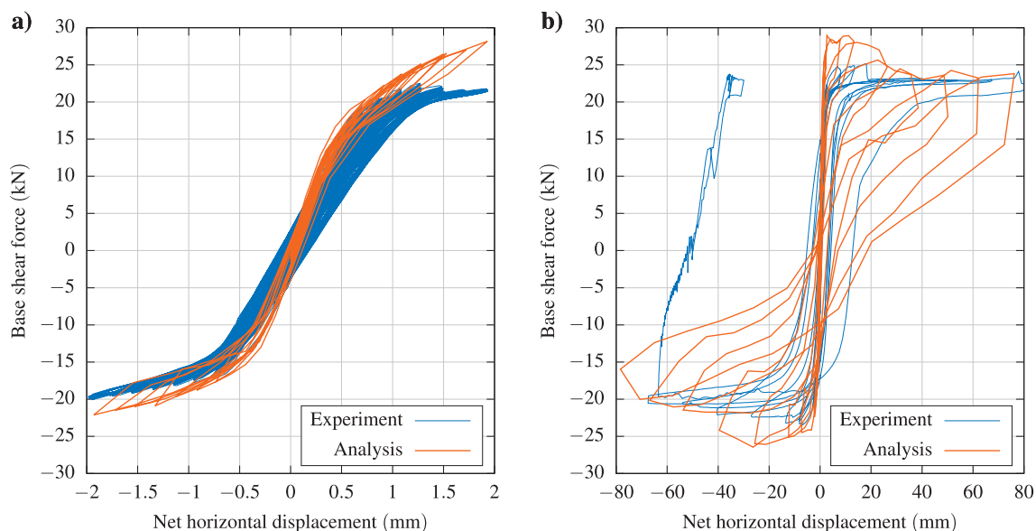
Fig. 9. Comparison of experimental and numerical force-displacement curves for a) phases 1 and 2, b) phase3.
