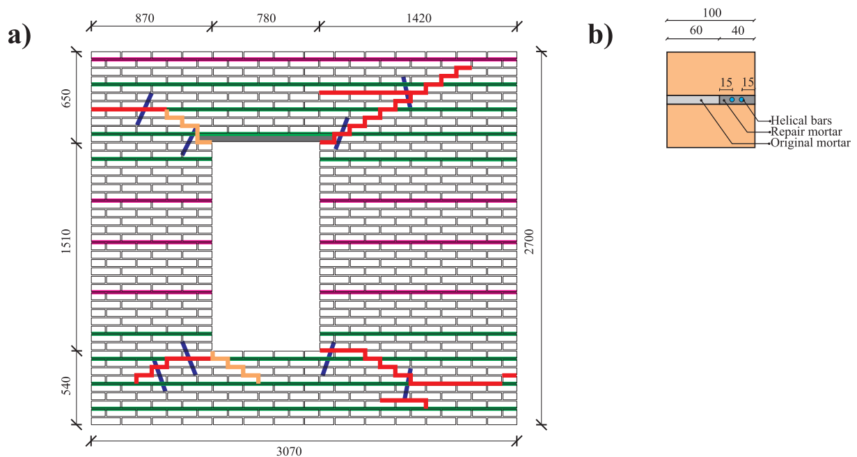
Fig. 3. a) Wall geometry, pre- and post-damage locations and strengthening layout: pre-damage in orange, post-damage in red, double bed joint bars in green, single bed joint bars in purple and single diagonal bars in blue. Positive loading direction towards right. b) Cross-section of repointed bed joint. All dimensions in mm.
