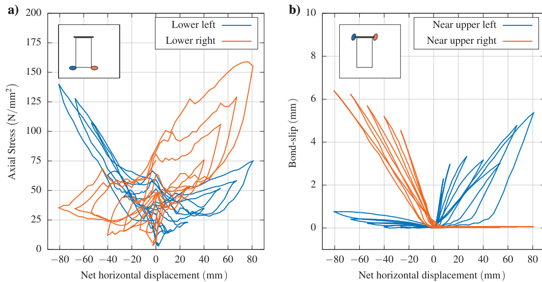
Fig. 11. Performance of reinforcement bars during phase 3: a) axial stress of bed joint bars near the base of the window, b) bond-slip of diagonal bars near the top of the window. Locations of measurements indicated in wall drawing insets.
