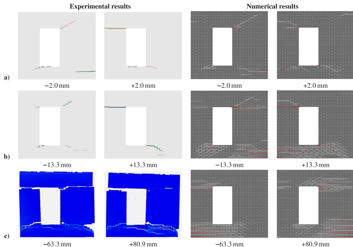
Fig. 10. Comparison of experimentally and numerically obtained (open cracks in red, closed cracks in white) cracking patterns for different levels of applied displacement: a) at the end of phase 2, b) near peak force and c) at the maximum applied displacement.
