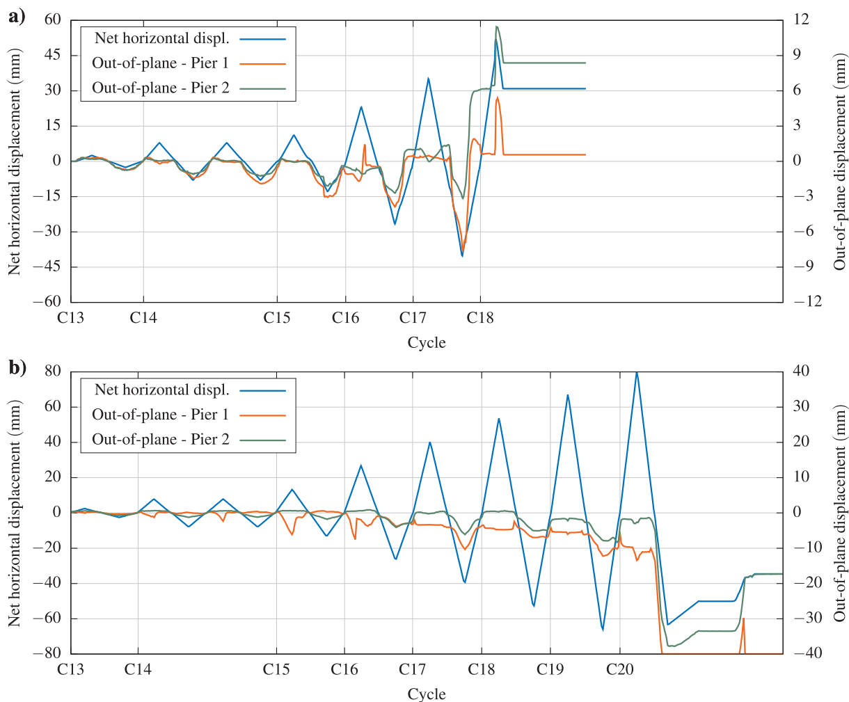
Fig. 7. Time-history of in-plane and of out-of-plane displacement of piers for a) unstrengthened and b) strengthened walls during phase 3.
