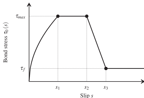
Fig. 8. Reinforcement bar bond-slip curve according to Model Code 2010.
