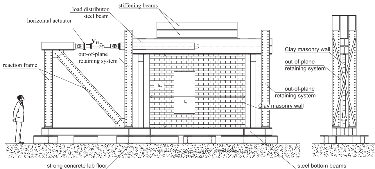
Fig. 1. Test setup for masonry wall in-plane testing.
