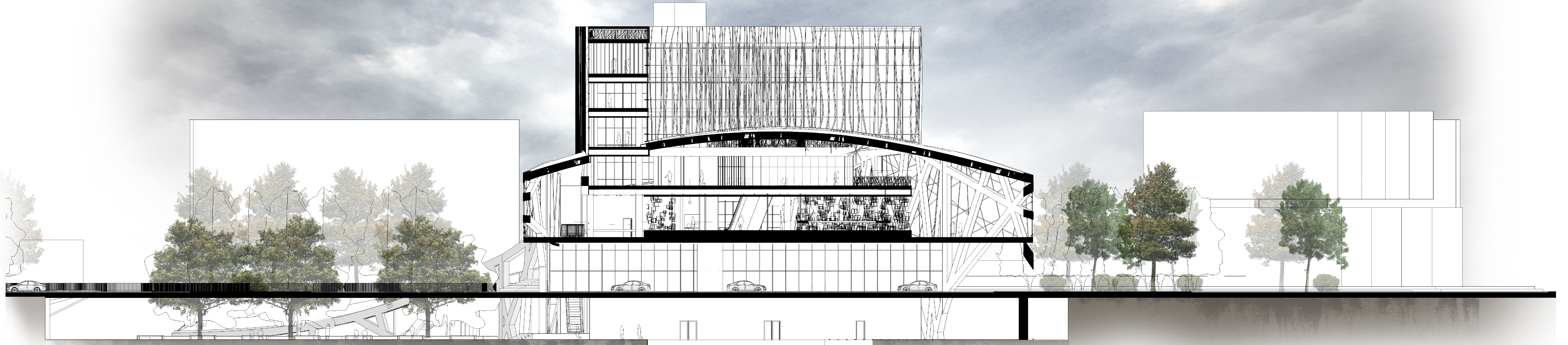
SECTION 1 scale 1:250
