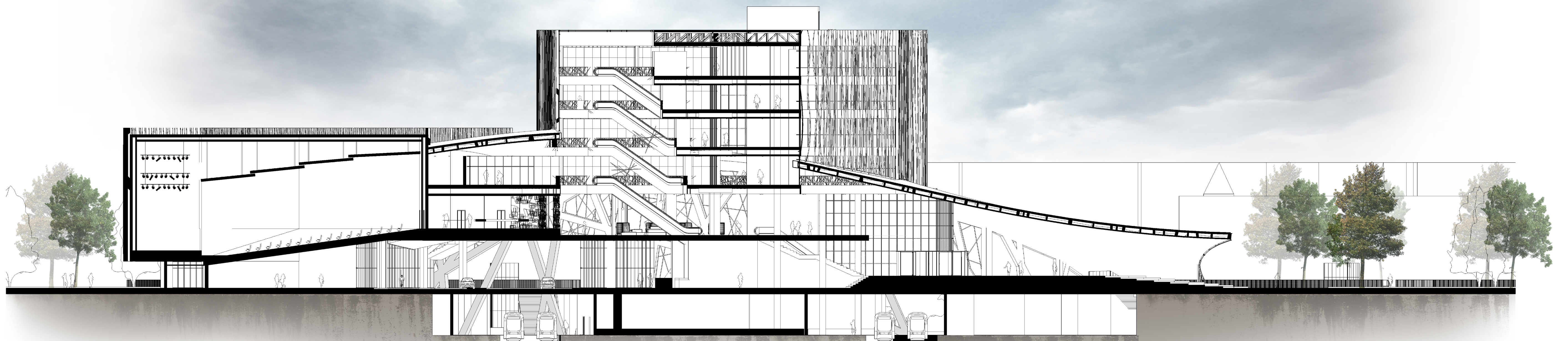
SECTION 3 scale 1:250
