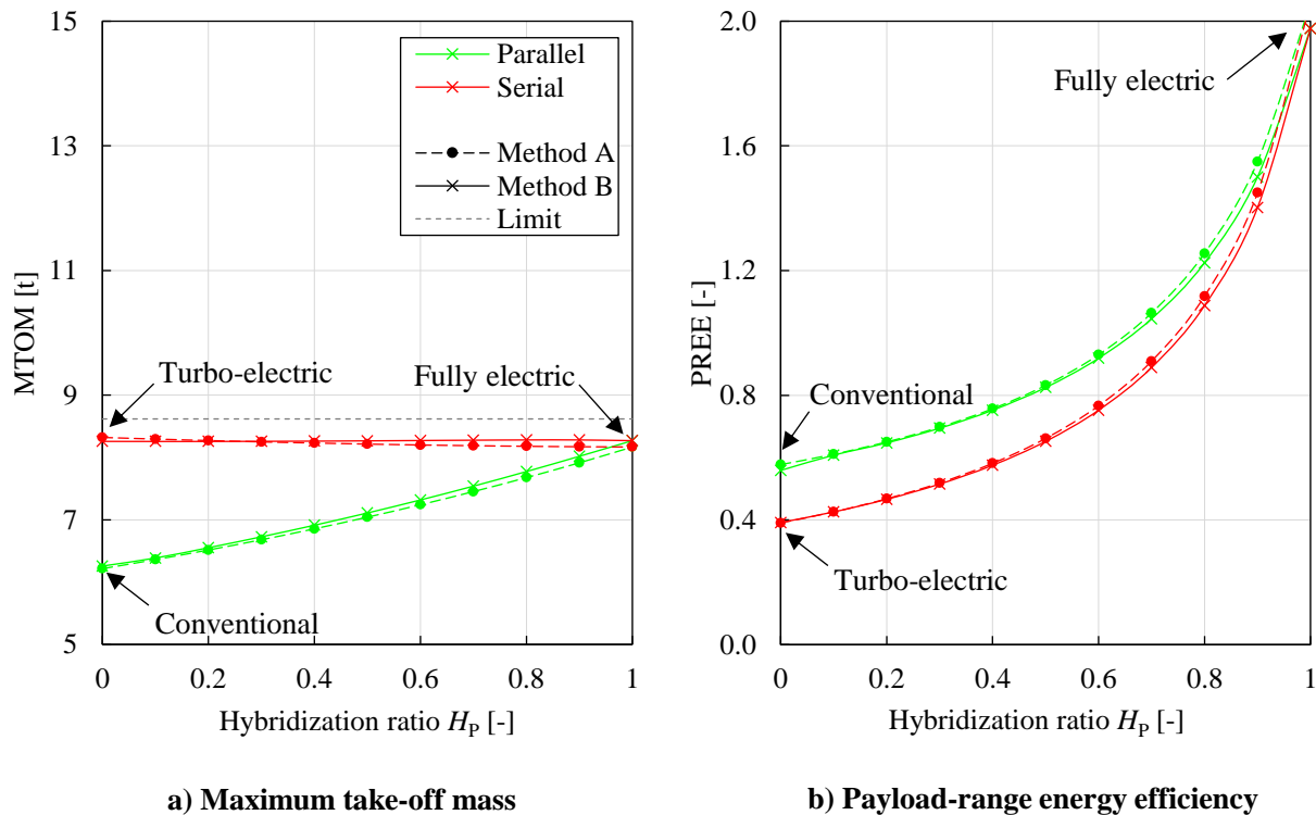
Fig. 15 Maximum take-off mass and PREE obtained for different hybridization ratios ( R = 396 km, E_{\text{bat}}^* = 1500 Wh/kg). The gray dashed line indicates the MTOM limit for a 19-passenger commuter aircraft per CS-23 regulations.
