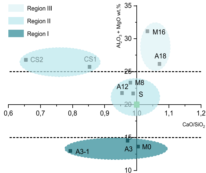
Fig. 14. (\text{CaO}/\text{SiO}_2) – (\text{Al}_2\text{O}_3 + \text{MgO}) coordinate system in weight percentage. For the weight composition of these synthesized slags, please see data in Table 1. The green square in the coordinate system represents slag containing CaO: 40%, SiO 2 : 40%, Al 2 O 3 : 10%, MgO: 10% by mass, and this chemical composition of slag is most commonly seen in the industry.
