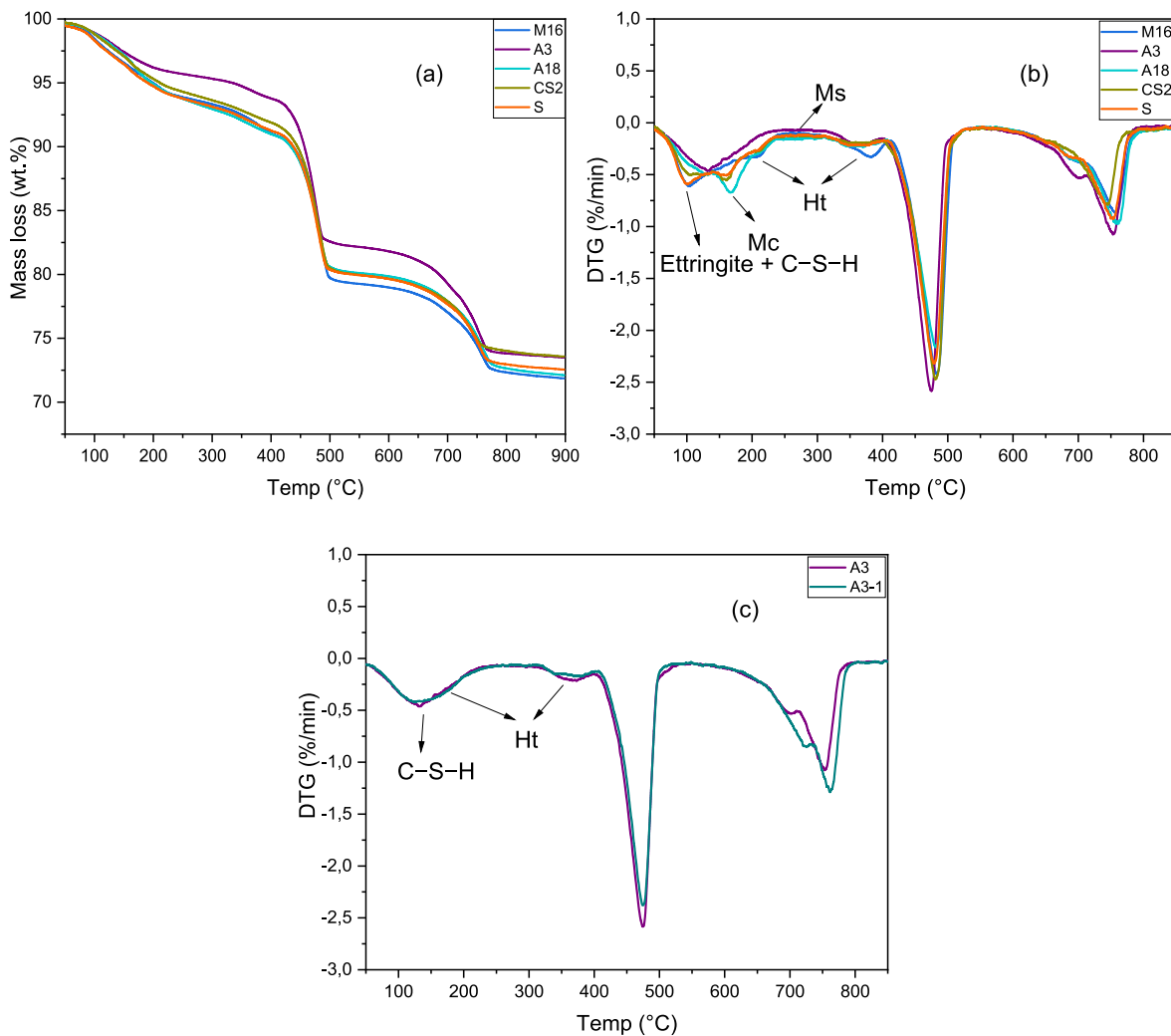
Fig. 7. Typical results of (a) TG and (b and c) DTG analyses of model pastes after 7 days curing at 40 °C. Ht: hydrotalcite-like phase; Mc: monocarbonate; Ms: monosulfate.
