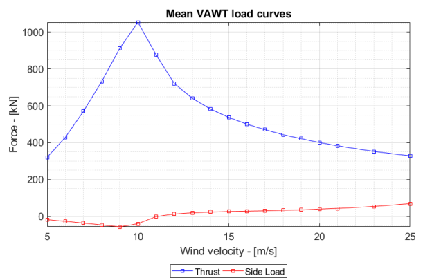
Figure 5. Thrust and side load curves
