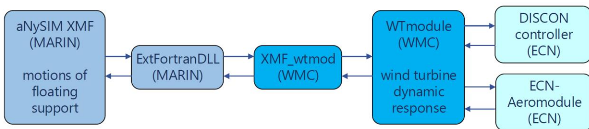
Figure 6. Coupled software for floating VAWT analysis
