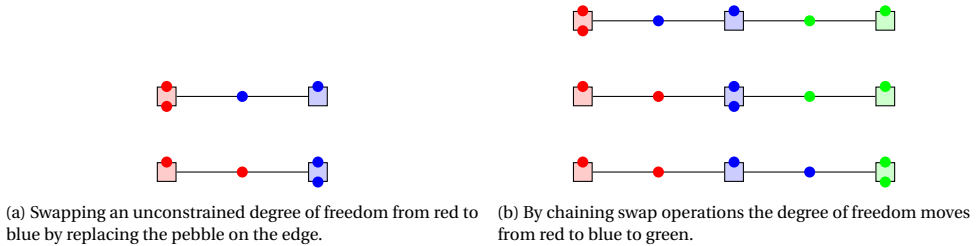
Figure 2.9: Degrees of freedom can move around a network by swapping the pebble that covers an edge repeatedly.
