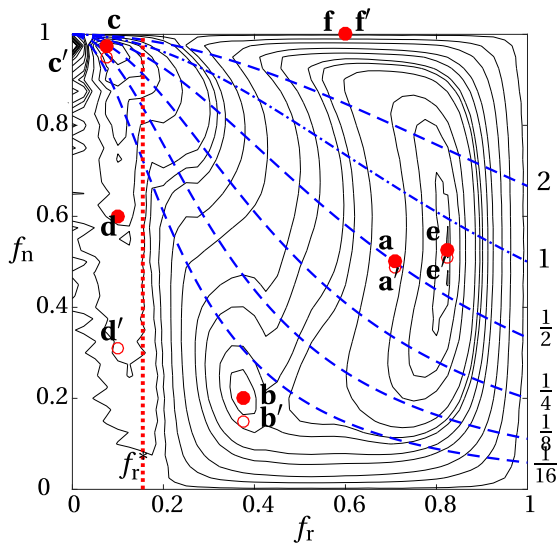
Figure 4.3: (a) \phi_c surface as a function of number and size ratio. (b) Contours of the same surface. The (dot-)dashed curves follow constant ratio of species volume (value indicated on the right). Voids in a triangle of large particles can hold at least one small rattler for f_r < f_r^* . Mixtures that are discussed are marked (see fig. 4.1); a prime denotes the shift of the point when using the corrected f'_n .
