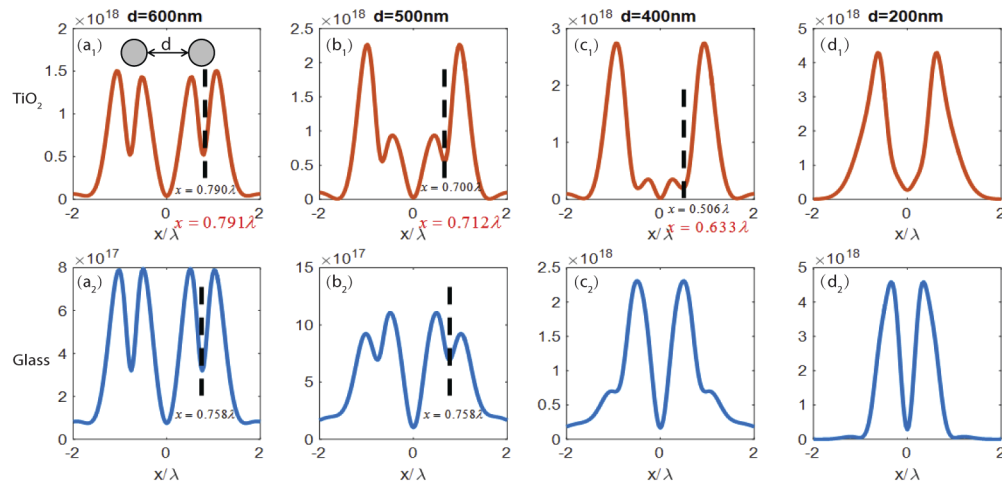
Fig. 6. Profile of the imaging of two separated nanospheres supported on different substrates with various distances between the spheres: d = 600nm , d = 500nm , d = 400nm and d = 200nm . (a 1 )-(d 1 ): with the enhancing TiO 2 slab on the top of glass, (a 2 )-(d 2 ): without enhancing slab.
