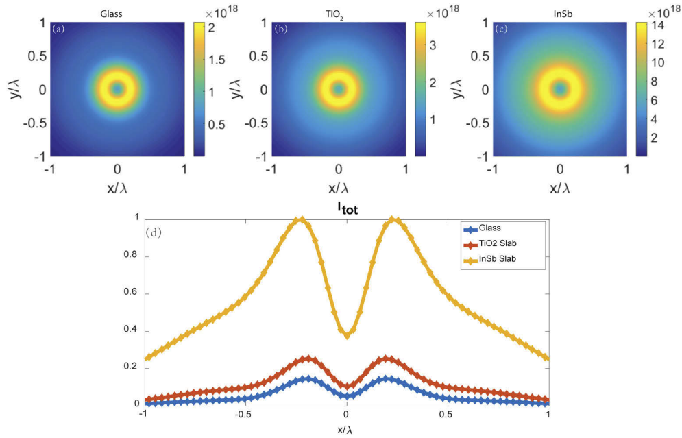
Fig. 5. Imaging of one sphere in the xy plane without (a) and with ((b)-TiO 2 , (c)-InSb) the enhanced layer under the illumination of radially polarized light. (d) is the cross section of the normalized scattering intensity.
