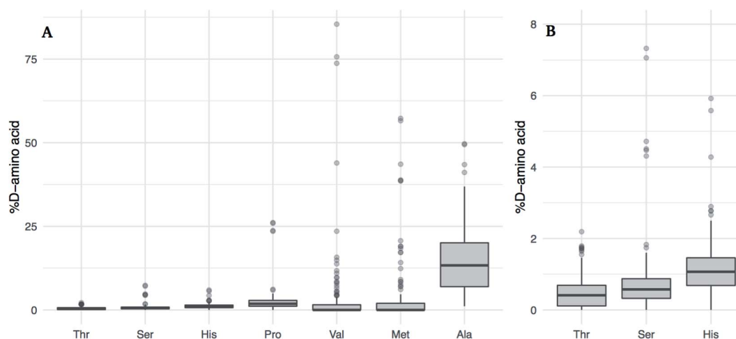
Fig. 3 (A) The percentage D-amino acid of threonine, serine, histidine, proline, valine, methionine and alanine in freshly deposited fingerprints of 40 donors. (B) Enlargement of the percentage D-amino acid of threonine, serine and histidine.
