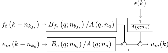
Fig. 4. Generic ARX model structure.
