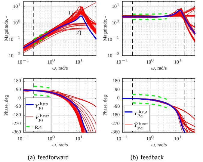
Fig. 11. Bode plots of \hat{Y}_p^{\text{best}} , SI-P ( c = 3 , K_{pt} = 0.3 ), other parameter values as given in Table I. Dashed lines indicate boundaries imposed by R.4, drawn for the frequency range over which R.4 is tested.
