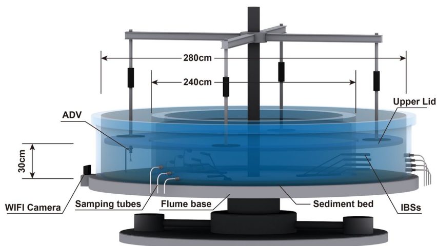
Figure 1. Overview of the annular flume and setup of instruments.
