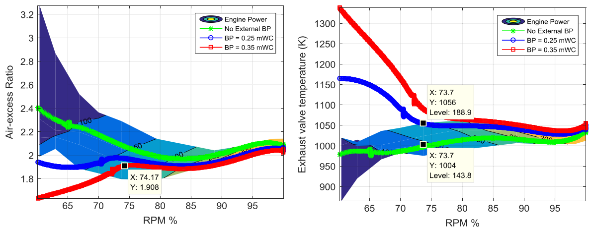
Fig. 5.4. Back pressure effect on air-excess ratio (a) and exhaust valve temperature of a constant pressure turbocharged engine, with 100 degree valve overlap.
