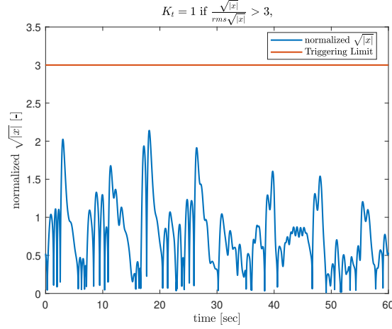
Fig. 18 Example normalized \sqrt{|x|} signal compared to the model's Triggering limit for DYN21, where the Triggering is not activated for the CE dynamics transition at 30 s.
