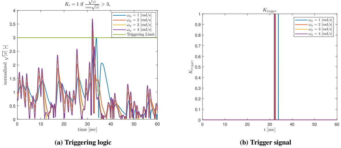
Fig. 11 The effect of varying the H(s) filter's break frequency \omega_{lp} in condition DYN12 on (a) the Triggering logic, and (b) the triggering signal K_{trigger}(t) .
