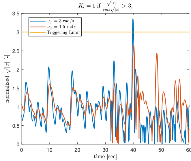
Fig. 15 Effect of increasing \omega_{lp} of the H(s) filter from 1.5 rad/s to 3 rad/s on the Triggering mechanism for Subject 00.
