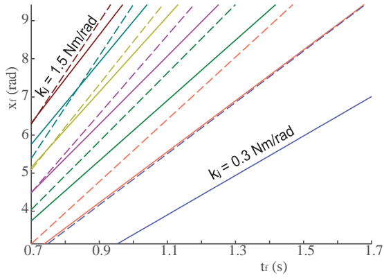
Figure 8. The optimal task manifold for nine different stiffnesses in simulation. The figure shows the manifold both from an idealized model (solid lines) and from simulations with a realistic model (dashed lines). It shows that the two models are comparable, especially at high stiffnesses.
