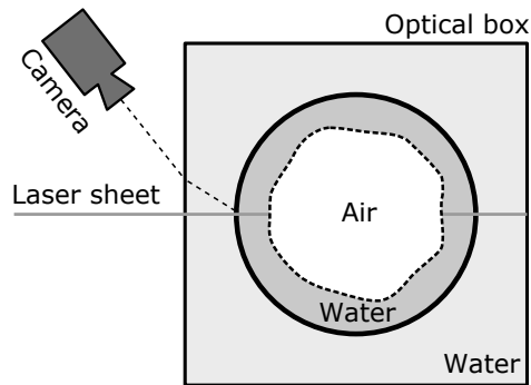
Figure 2.3: Schematic of the PLIF set-up used in the visualization measurements, as seen from the top. The water in the interior of the pipe is dyed with 125 \mu\text{g}/\text{L} rhodamine, water in the optical box with 50 \mu\text{g}/\text{L} .
