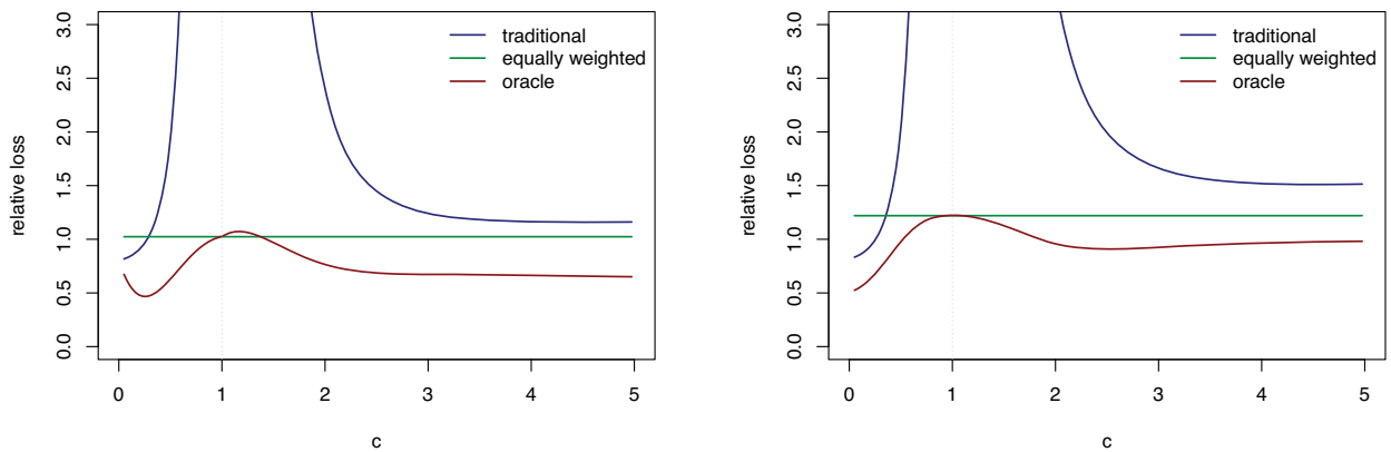
Figure 4. The relative losses for the portfolios based on the optimal shrinkage estimator, the traditional estimator and the equally weighted portfolio as a function of c for the calibration criteria (i)-(ii) from Proposition 2.1 (left to right). The dimension is set to p = 100 and the condition index is set to 1000.
