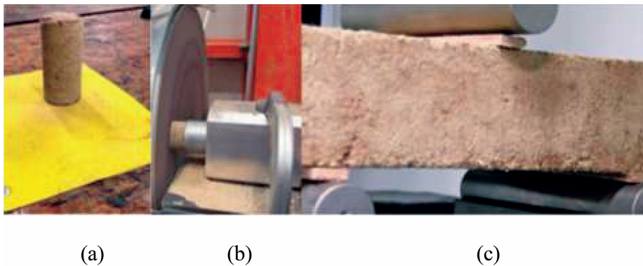
FIGURE 4. Sanding paper (a) and machine (b) used for rectification purposes and wooden strip interposition between steel rolls in a three point bending test (c) [24], [33.]
