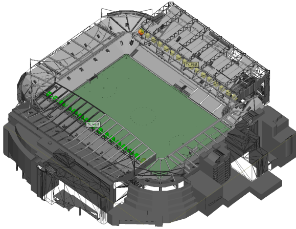
Fig. 3: Football stadium 3-D model
