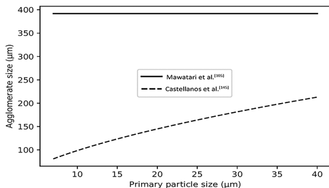
FIGURE 6 Predicted agglomerate size versus primary particle size; using parameters for hydrophobic SiO 2 : A_H = 1.5 \cdot 10^{-19} J, z_0 = 4 \cdot 10^{-10} m, D_a = 2.5 , d_{asp} = 2 \cdot 10^{-7} m, \rho_p = 2560 kg/m 3 , \rho_a = 55 kg/m 3 , \rho_f = 1.25 kg/m 3 , g = 9.81 m/s 2 , u_{cha} = 5 \cdot 10^{-3} m/s, \varepsilon_{cha} = 0.75 , H_f = 10^8 N/m 2
