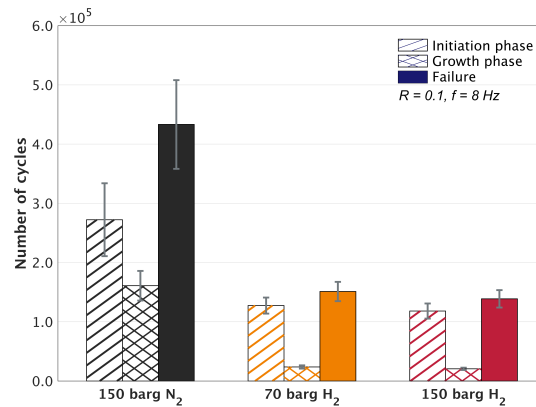
Figure 6. Bar graph of the number of cycles spent in the crack initiation phase ( N_I ) and the growth phase ( N_G ), and the total number of cycles until failure ( N_F ) of the weld metal specimens. The different environments tested are shown with distinct colors. The single and double hatched bars represent the number of cycles spent in the initiation and growth phase, respectively. Error bars are standard deviations.
