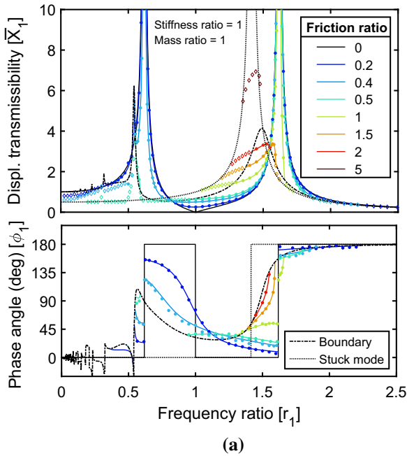
Fig. 11 Displacement transmissibilities and phase angles of a 2DOF system with a contact on m_2 and a harmonic load on m_1 for varying friction ratios and unitary mass and stiffness ratios, displayed on m_1 (a) and on m_2 (b). Analytical results are represented by the continuous lines, while numerical results are
