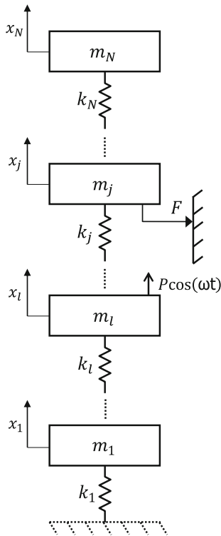
Fig. 1 MDOF system with a friction contact on the j th mass subjected to a harmonic excitation on the l th mass
