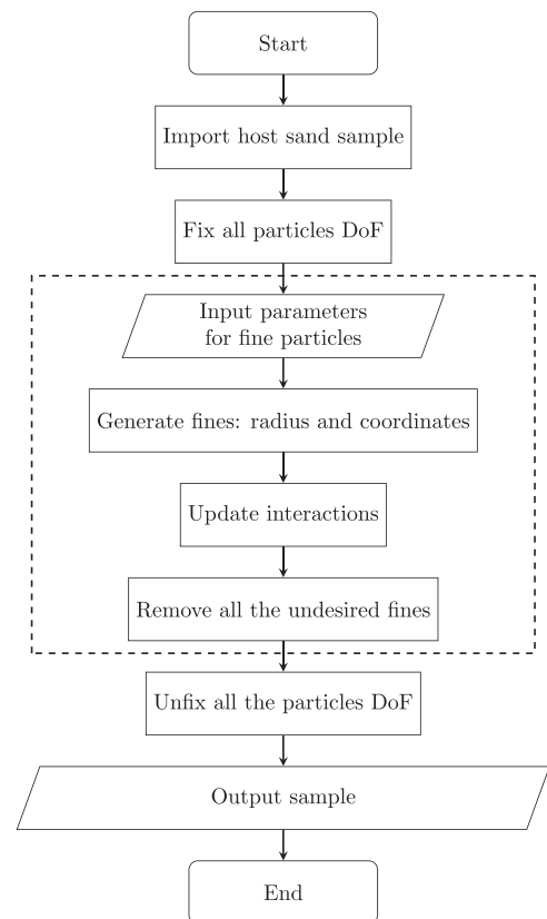
Fig. 2. Flowchart for generating samples containing fines with various microstructures.
