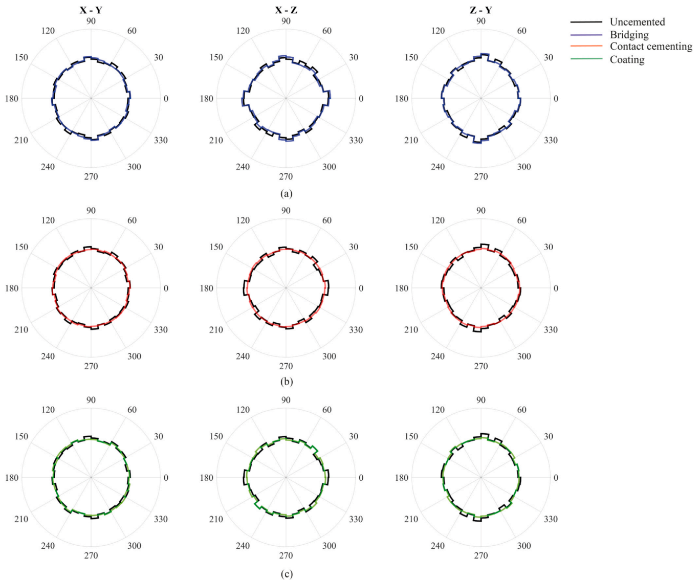
Fig. 7. Contact normal distribution of all inter-particle contacts: (a) bridging; (b) contact cementing; (c) Coating. The contact normal distribution of the uncemented sample is also plotted in each figure.
