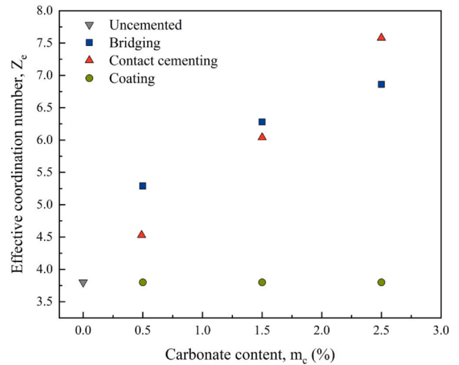
Fig. 6. Effective coordination number of uncemented sample and bio-cemented samples with different carbonate distribution patterns and contents.
