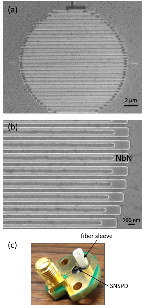
Fig. 2. (a,b) SEM images of the NbN meander. (c) SNSPD device mounted on a print circuit board for characterization.
