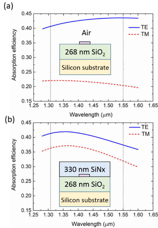
Fig. 3. Calculated absorption efficiency as a function of the wavelength (a) for the uncapped NbN meander; (b) for the NbN meander covered with 330 nm of \text{SiN}_x . Insets: Designs of the structures for which simulations have been performed.
