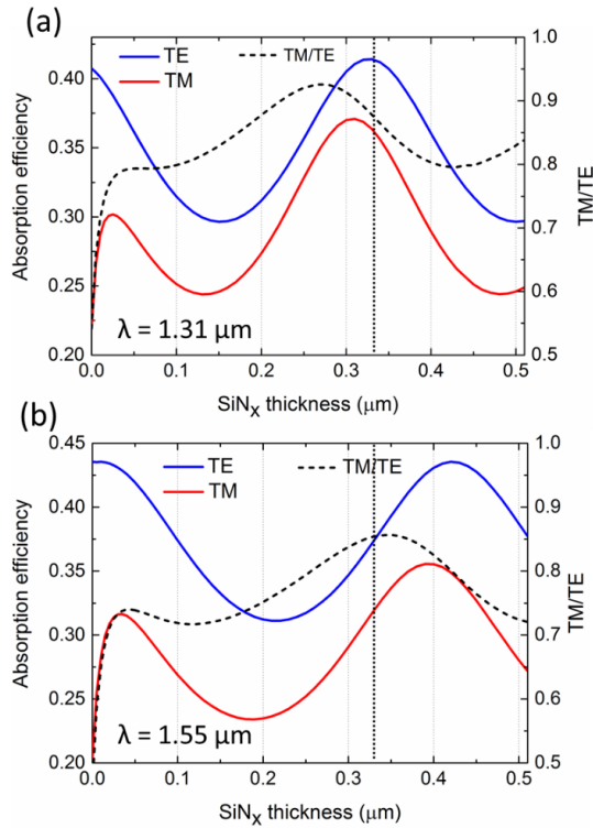
Fig. 4. Calculated dependence of TE and TM absorption efficiency, as well as the TM/TE absorption ratio, as a function of the thickness of the SiN x cap layer at (a) 1.31 μm, and (b) 1.55 μm.
