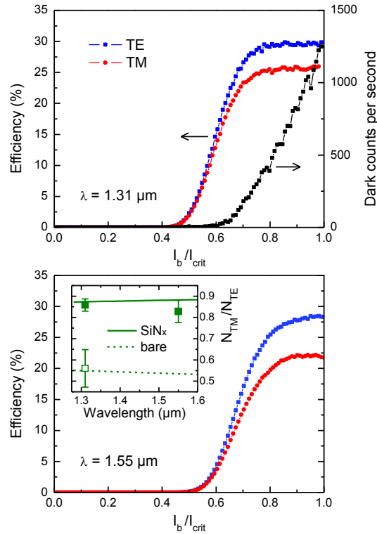
Fig. 5. Detection efficiency as a function of the bias current / critical current ratio ( I_b/I_{\text{crit}} ), measured for a typical SNSPD device (a) at 1.31 \mu\text{m} , and (b) at 1.55 \mu\text{m} . The dark count rate is represented in (a). Inset in (b): measurement of the N_{\text{TM}}/N_{\text{TE}} response ratio of bare devices (open symbol) and devices capped with SiN x (solid symbols). The curves represent theoretical calculations for both cases.
