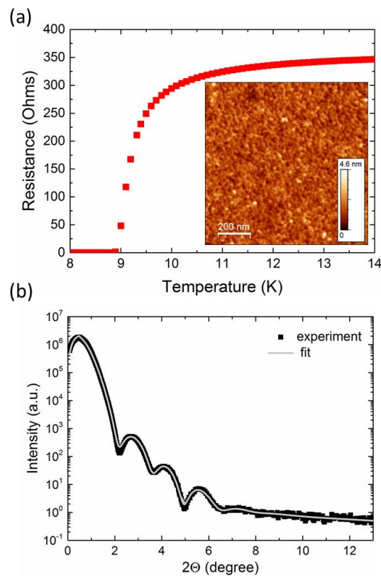
Fig. 1. (a) Film resistance vs. temperature for the NbN thin film under study. Inset: 1 \times 1 \mu\text{m}^2 atomic force microscopy image of the NbN surface. (b) X-ray reflectivity of the NbN film on SiO 2 -on-silicon. Black squares are experimental measurements and the solid gray line is a fit generated with the GenX software.
