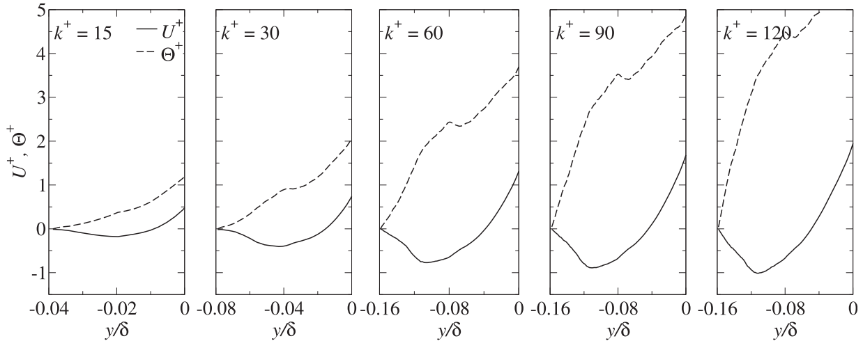
Fig. 13. Velocity and temperature profiles well within the roughness sublayer.
