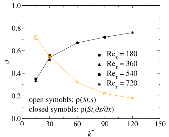
Fig. 17. Correlation coefficients \rho(s, St) and \rho(\partial s / \partial x, St) .
