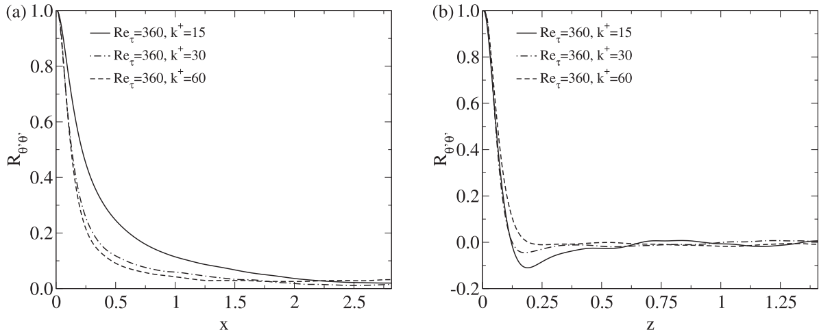
Fig. 3. (a) Autocorrelation function R_{\theta^i \theta^j} at y^+ = 15 as a function of the streamwise coordinate x . (b) Autocorrelation function R_{\theta^i \theta^j} at y^+ = 15 as a function of the spanwise coordinate z .
