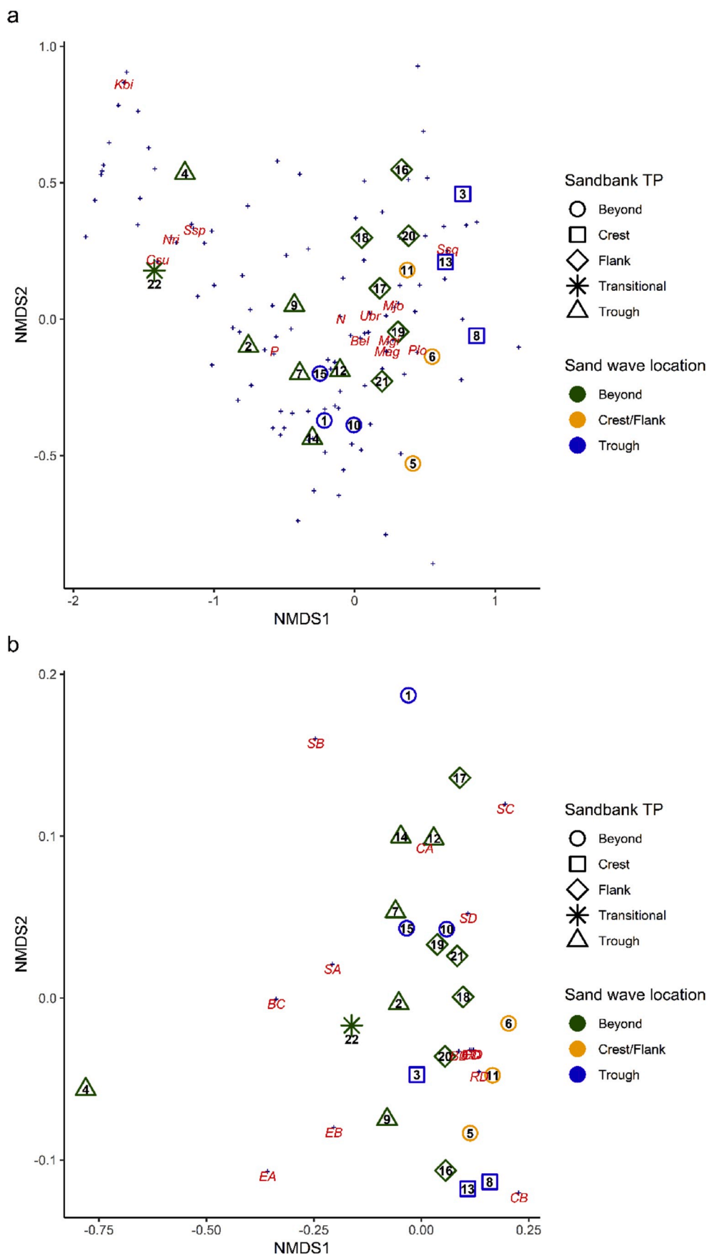
Fig. 2. NMDS plots based on (a) taxonomical composition of the macrobenthic communities, with indication of the species that contributed more than 5% to the dissimilarity between topographic positions (TP) in the SIMPER analysis ( Bel : Bathyporeia elegans ; Csu : Callianassa subterranea ; Kbi : Kurtiella bidentata ; Mag : Megaluropus agilis ; Mgi : Monopseudocuma gilsoni ; Mjo : Magelona johnstoni ; N : Nemertea; Nri : Nephasoma rimicola ; P : Phoronis sp.; Plo : Pseudocuma longicorne ; Ssp : Sabellaria spinulosa ; Ssq : Scolecipis squamata ; Ubr : Urothoe brevicornis ) and (b) functional composition of the macrobenthos communities, with functional groups based on sediment reworking mode (E: epifauna, S: surficial modifiers, C: conveyor-belt feeders, B: biodiffusors, R: regenerators), and motility in the sediment (A: in a fixed tube; B: sessile, but not in a tube; C: slow movement through the sediment; D: free movement through a burrow system).
