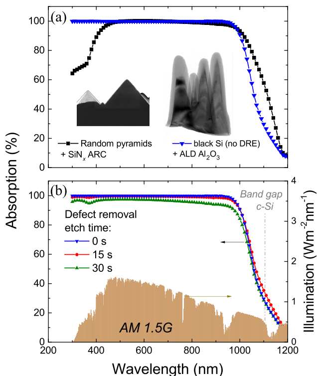
FIG. 2. (a) Absorption in 280 \mu\text{m} thick c-Si with either a b-Si front surface texture which was passivated by 30 nm of ALD Al 2 O 3 or a random-pyramid texture and a 75-nm SiN x anti-reflection coating. The inset shows scanning and transmission electron microscopy images of the surface textures (not to scale). (b) Absorption of b-Si, passivated by 30 nm of Al 2 O 3 , for various defect removal etching (DRE) times. Additionally, the AM1.5 spectrum is displayed for reference.
