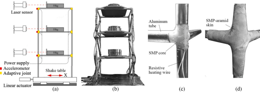
Fig. 5. (a) Experimental setup; (b) three-story adaptive frame prototype; (c) SMP core connected to four aluminum tubes; (d) SMP-aramid skin.
