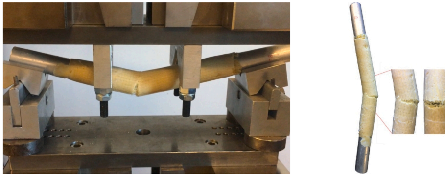
Fig. 19. Specimen B2 failure under four-point bending test at 25 °C.
