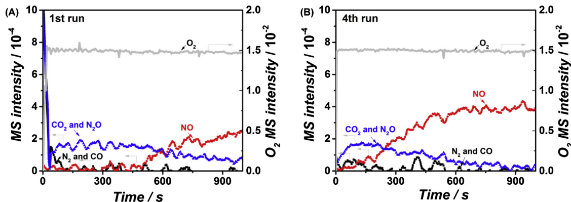
Fig. 7. Gasses evolution during exposure of Rh/K/CZ C 3 H 6 reduced at 400 °C to a 0.2% NO + 5% O 2 containing He flow at a GHSV of 67,000 l/h at 400 °C. (A) 1st cycle of NO and (B) 4th cycle of NO experiments.
