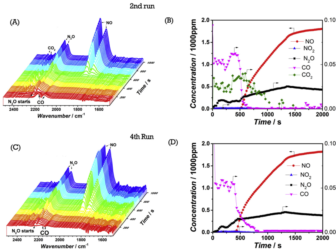
Fig. 5. Gasses evolution from the exit of the reactor: (A) and (C) FT-IR spectra; (B) and (D) are the quantitative data from (A) and (C), respectively. (A) and (C) were obtained during the 2nd and 4th NO experiment, respectively. Both experiments were performed at the conditions of 0.2% NO/He gas stream over an used Rh/K/CZ pre-treated by C 3 H 6 at 450 °C, GHSV of 67.000 L/L/h.
