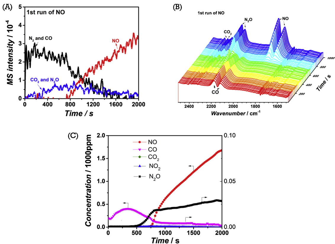
Fig. 4. Gasses evolution from the exit of the reactor: (A) MS signal; (B) FT-IR spectra; (C) the quantitative data from (B). The experiments were performed at the condition of 0.2% NO/He gas stream over fresh Rh/K/CZ pre-treated by C 3 H 6 at 450 °C, GHSV of 67.000 L/L/h.
