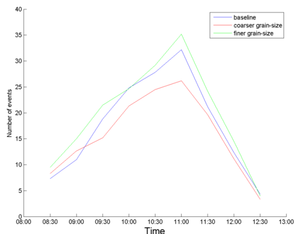
Figure 7. Average number of events for each time-step of the baseline model and the different grain-sizes models.
