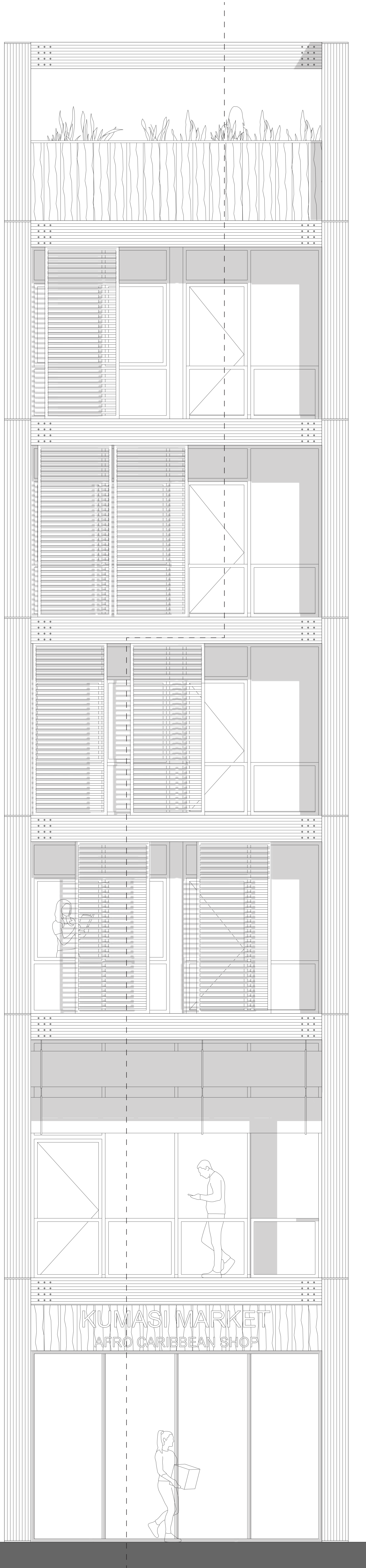
Facade Elevation Scale 1/20
