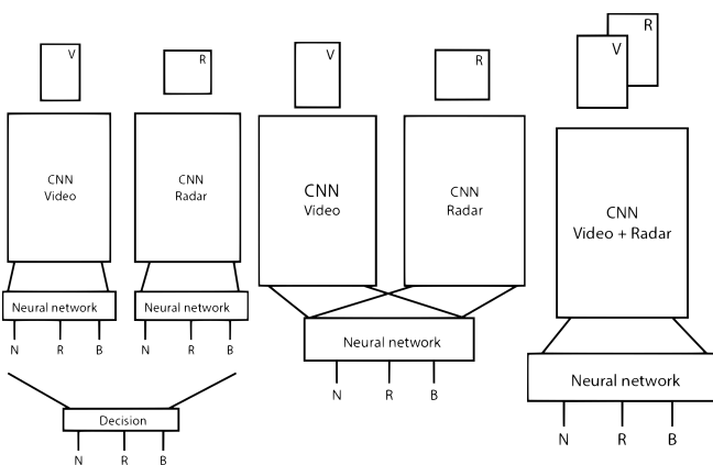
Fig. 1. Schematic block diagrams of three multimodal fusion approaches. Here “CNN” indicates the convolutional and pooling layers of the CNN used for feature extraction, whereas “Neural network” refers to the fully connected layer(s) (including a softmax layer) used for the final classification. The three output classes are denoted by “N,” “R,” and “B.”
