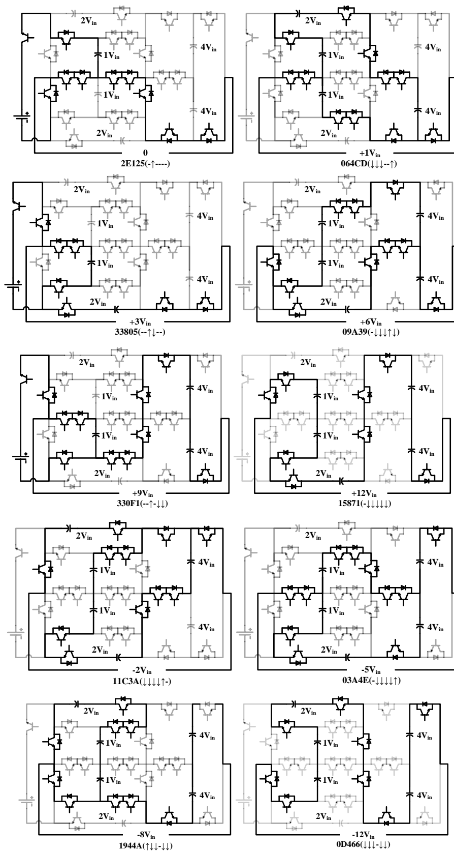
Figure 4. A few selected discharging paths related to the switching states of Table 1.
