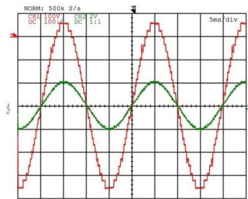
(b) CH1: 100 V/div, CH2: 2 V/div, 5 ms time/div
