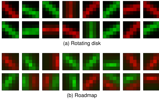
Fig. 9. SS-Conv kernels learned from real sequences. Synaptic strength is encoded in color brightness.
