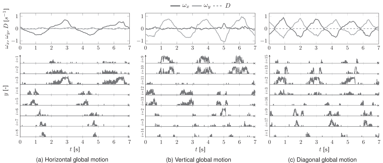
Fig. 13. Temporal course of the postsynaptic trace (as in Appendix D.4, available in the online supplemental material) of the eight most-active neurons (for each case) from the Dense layer learned from the roadmap texture (bottom), in response to different global planar motion patterns (top). Plots are normalized by the maximum trace on the stimuli evaluated: 1.0 by i = 3 at t = 3.0 s for the horizontal motion case. Optical flow visual observables ( \omega_x , \omega_y , D ) computed from the event sequences with the planar optical flow formulation from [55] (see Appendix C, available in the online supplemental material).
