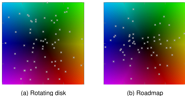
Fig. 10. MS-Conv kernels learned from real sequences in the (normalized) optical flow space, as in Appendices D.5 and D.6, available in the online supplemental material. Motion direction is encoded in color hue, and speed in color brightness. Each kernel is depicted as a cross.
