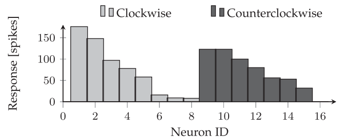
Fig. 11. Neural activity of the Dense layer trained in the rotating-disk sequence, in response to the two global motion patterns in this recording.
