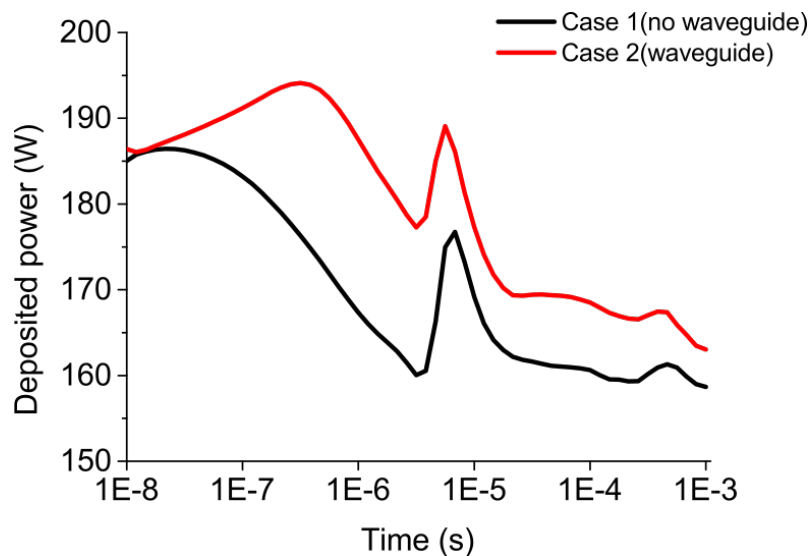
Fig. 3. Deposited microwave power over time for Case 1 (no waveguide) and Case 2 (waveguide).
