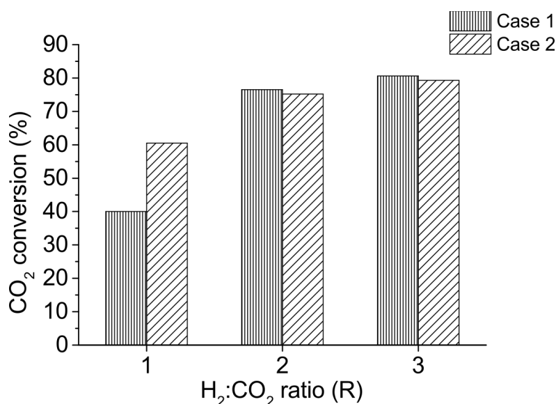
Fig. 6. Comparison of CO_2 conversion for two MWP reactor configurations: Case 1, extended waveguide not included; Case 2, extended waveguide included. Operating conditions: total gas flow rate = 0.4 l/min, net input microwave power = 150 W, operating pressure = 25 mbar.
