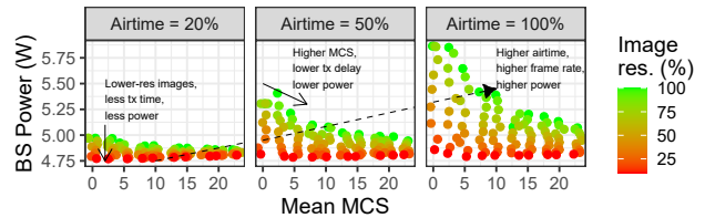
Figure 5: BS power consumption vs. radio policies for images with different resolutions.
