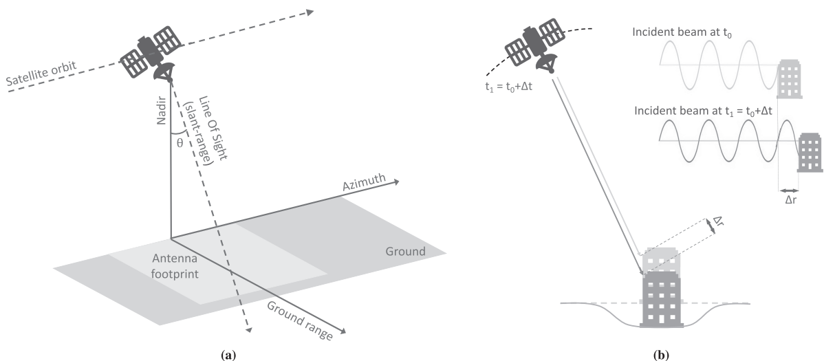
FIGURE 2 (a) Simplified satellite InSAR acquisition geometry. (b) Simplified sketch of the InSAR capability to measure building deformations
