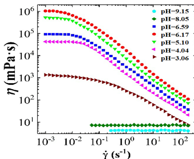
Figure 11. The steady rheological curves for the CTAB-CA based (30 mM CTAB + 15 mM MA) VES-fluid at pH range ( 3 < \text{pH} < 10 ) and at 25 °C.
