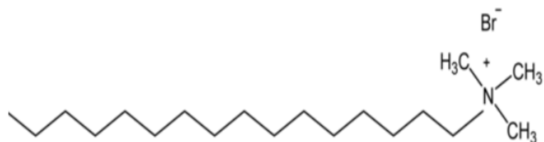
Figure 3. Chemical structure of CTAB.
