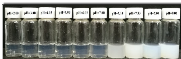
Figure 8. Phase behaviour of CTAB-MA solution at different pH values.
