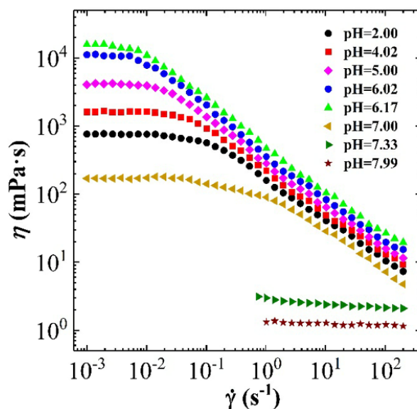
Figure 12. The steady rheological curves for the CTAB-MA based (30 mM CTAB + 15 mM MA) VES-fluid at pH range ( 2 \leq \text{pH} < 8 ) and at 25 °C.
