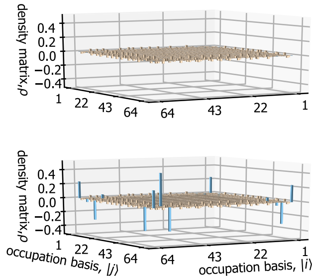
FIG. 11. Reduced density matrix. In the upper panel, we show the case with eliminated edge-edge component; in the lower panel, we show the case with eliminated bulk-bulk components. The edge-edge components are highlighted in light blue color.
