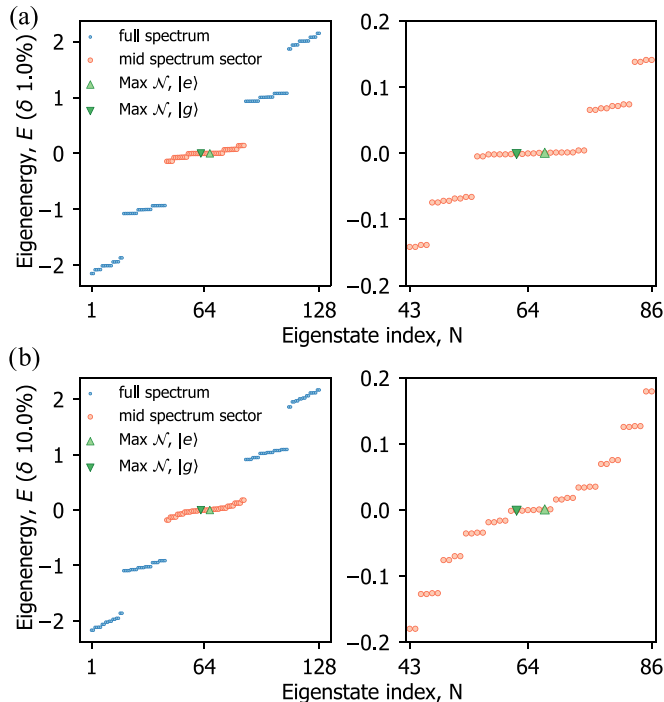
FIG. 5. (a) Eigenenergy spectrum with \delta = 1\% . (b) Eigenenergy spectrum with \delta=10\% . Both are in the topological regime ( v=0.1 , w = 1.0 ). The two green upward and downward triangles represent the two maximally entangled states when the qubit is projected to |e\rangle or |g\rangle , respectively. The middle near-zero-energy section in the spectrum (highlighted in orange) is enlarged in the right panel.
