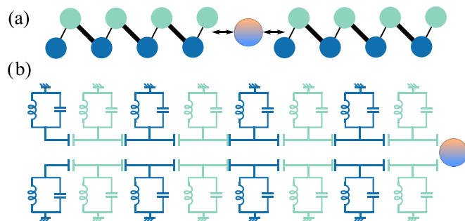
FIG. 2. (a) Schematic plot of two SSH arrays coupled to one qubit, each chain consisting of four unit cells of two sublattice sites. Blue and green colors represent the A and B types of sublattice. The orange-blue gradient circle represents the qubit. Arrows represent dispersive coupling between the qubit and the edge lattice sites. (b). Each sublattice site represents one superconducting LC resonator. The varying capacitive coupling between resonators is indicated with the capacitor distance.
