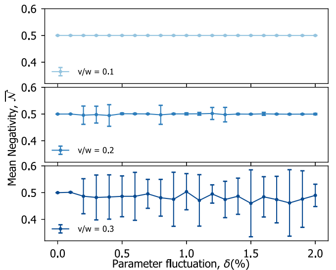
FIG. 7. Mean negativity \overline{\mathcal{N}} as a function of parameter fluctuation strength \delta under different v/w ratios. The mean negativity is calculated from all states with eigenenergy in the energy window. Each point represents the mean negativity value with the standard deviation indicated by the error bar. Each data point is calculated from 100 randomly sampled Hamiltonians under the specific \delta .
