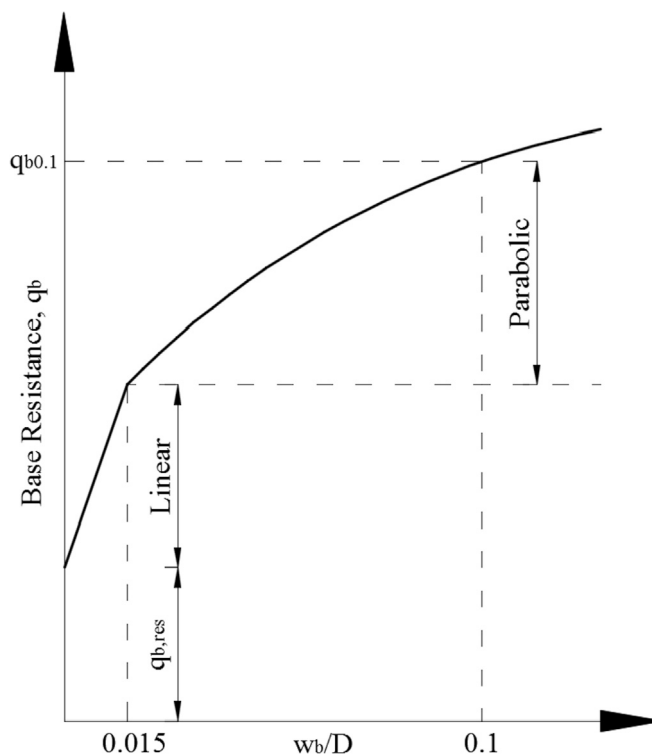
Fig. 4. Base resistance-settlement model.
