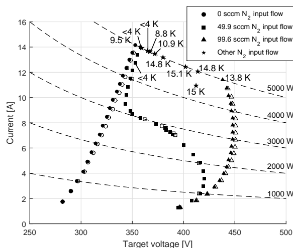
Fig. 3. LLS801 I - V relationships in the high flow regime. The argon input flow is 400.8 sccm and the argon partial pressure 0.7 Pa. Deposited thin films have an added T_c value. Isopower curves are depicted by the dashed lines. Upward power sweeps are indicated by the filled symbols, downward power sweeps by the unfilled symbols.
